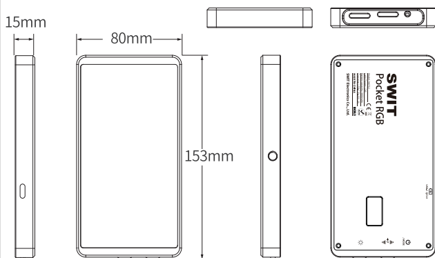
Fig. 1 S-2712 Overall Dimension
